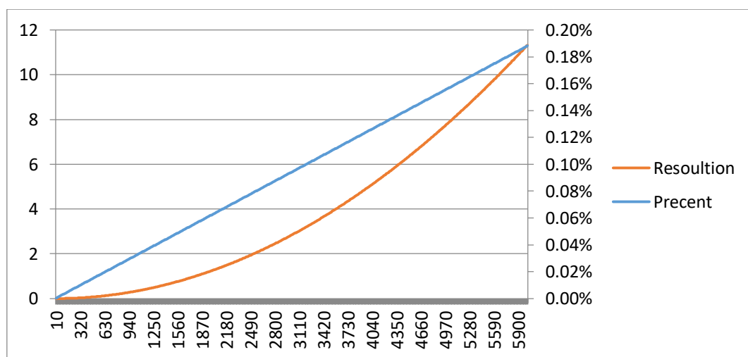
Figure 2-2 The Trend Graph of RPLIDAR A1 Resolution
