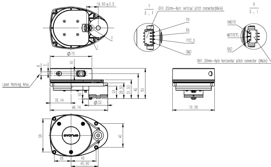
Figure 5-2 The Mechanical Dimensions of RPLIDAR A1
